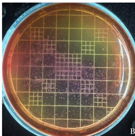
Figure 1. (A) Opaque yellow colonies with entire margin. (B) Translucent red to pink colonies with punctiform shape.
